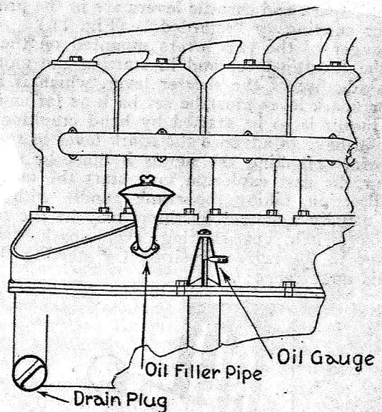
Fig. 6—Gauge must show lubricant in crankcase (Model 71)
